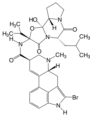
(11) Bromocriptine
