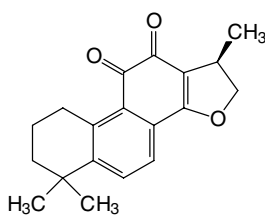
(65) Cryptotanshinone
