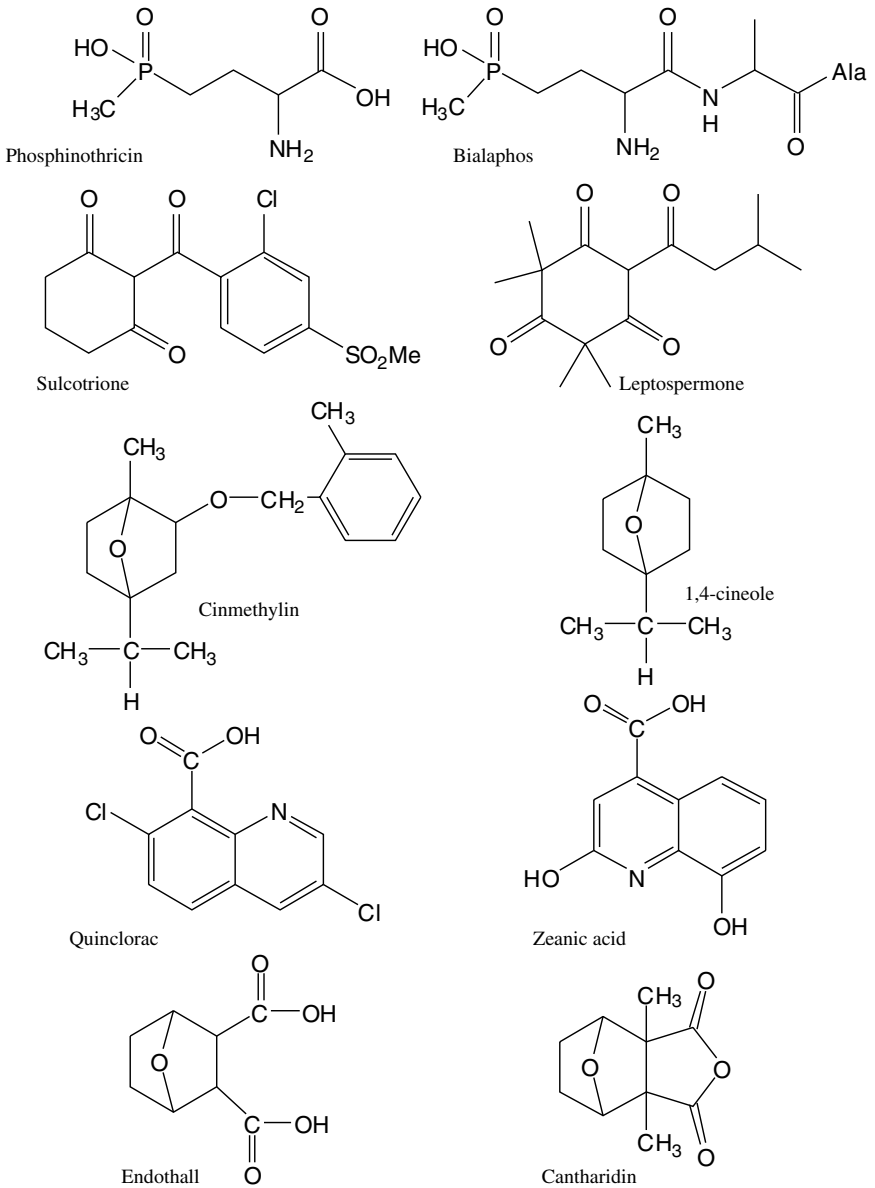
Fig. 20. Structures of commercial herbicides and their natural product analogues.
