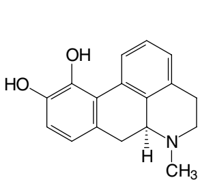
(15) Apomorphine
