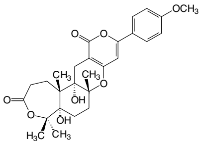
(80) Isoterreulactone A
