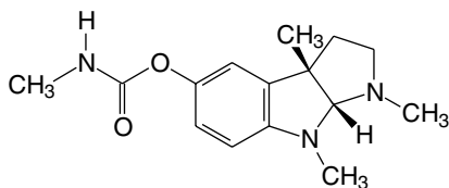
(33) Physostigmine
