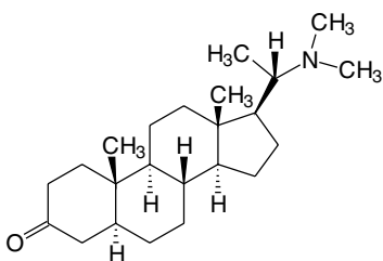
(51) Buxakashmiramine
