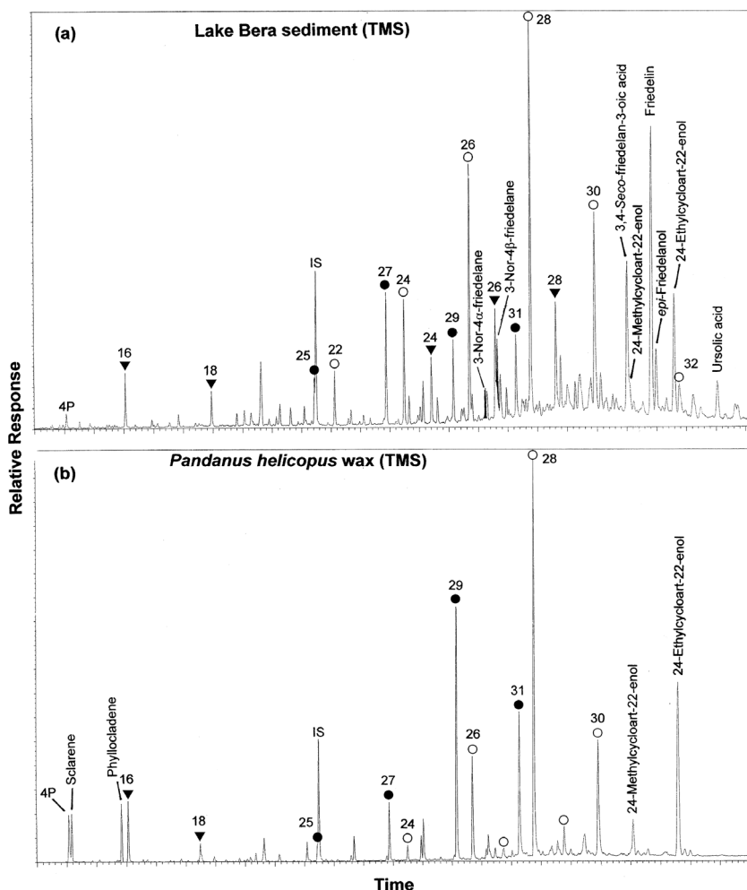
Fig. 10. GC-MS TIC traces for total extracts of: (a) a tropical lake sediment, and (b) epicuticular wax from a dominant reed growing in the shallow areas of the lake (analyzed as TMS). Numbers and symbols as in Fig. 9, 4P = dibutyl phthalate contaminant, IS = internal standard.
