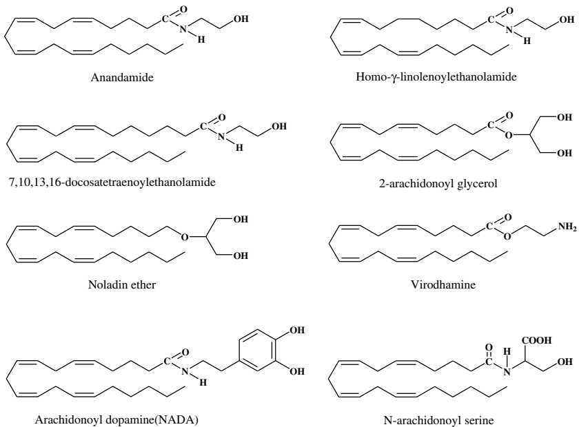
Fig. 3. Structures of most known endocannabinoids.
